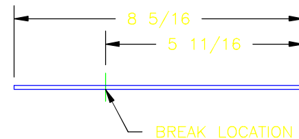
BREAK DETAIL CUT SIZE: 8-5/16x48
