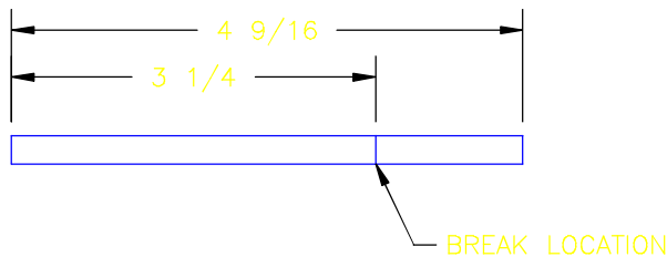
ITEM B MATL: FI 1/4 x 1 x 4-9/16 HRS 1 REQUIRED
