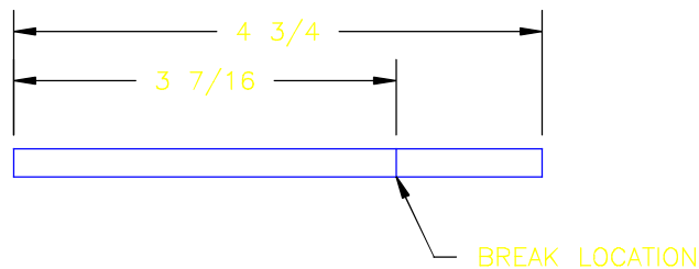
ITEM A MATL: FI 1/4 x 1 x 4-3/4 HRS 1 REQUIRED
